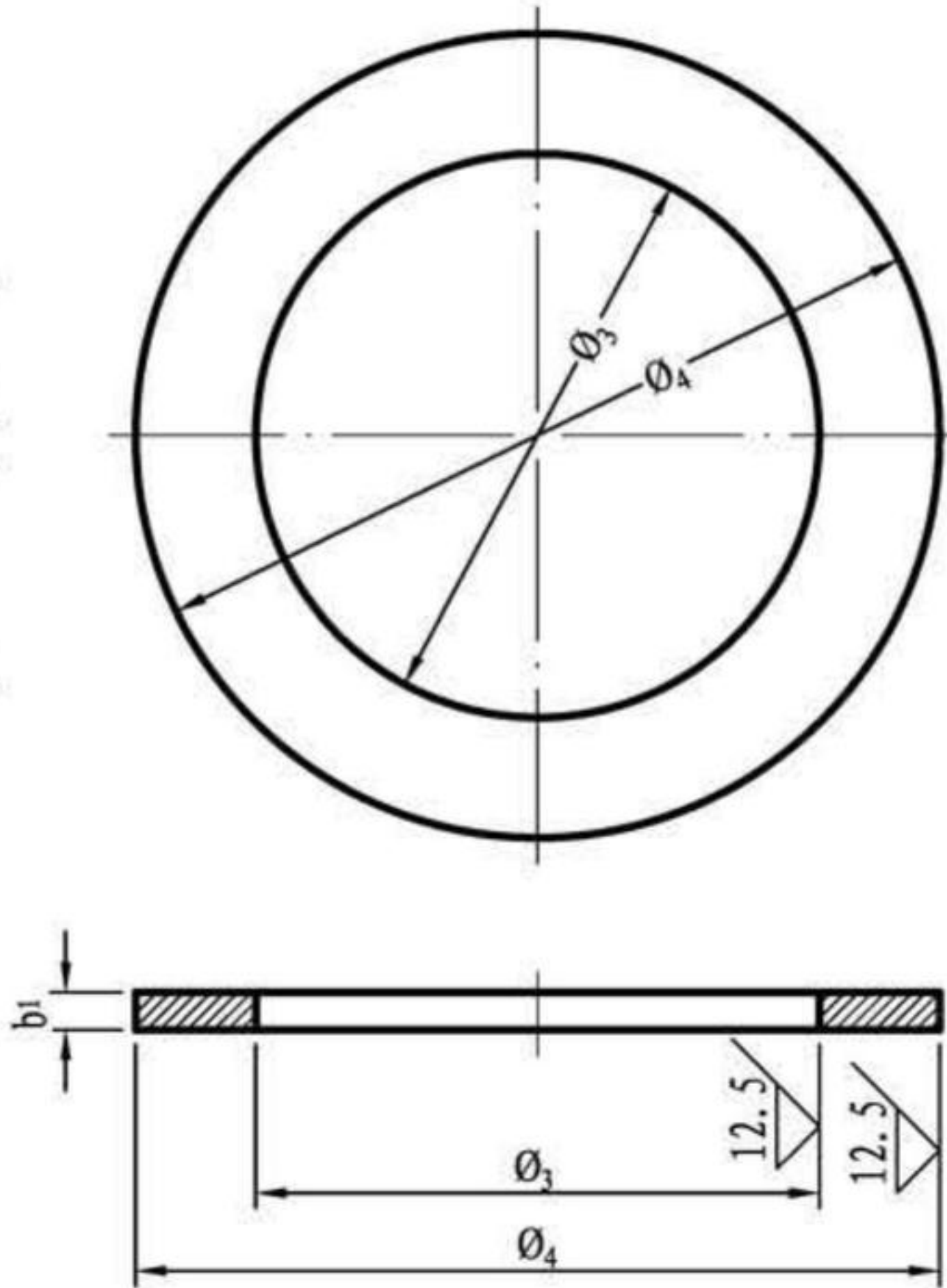
翼环
