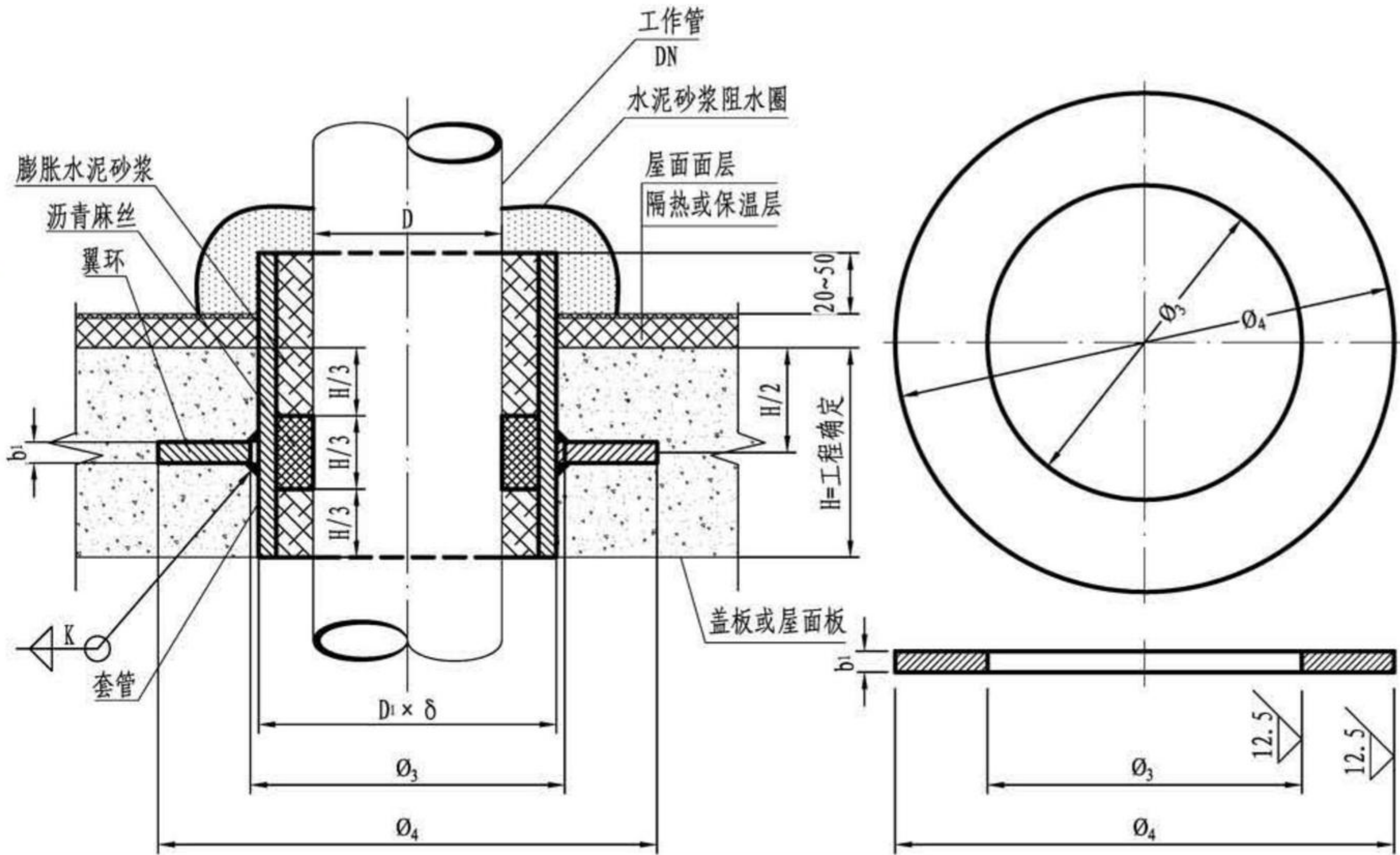
翼环
