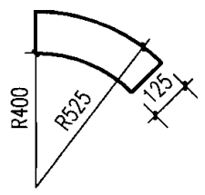
C30预制混凝土砌块大样
