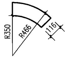
C30预制混凝土砌块大样
