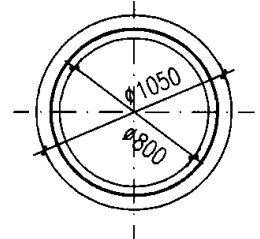
预制井筒大样
