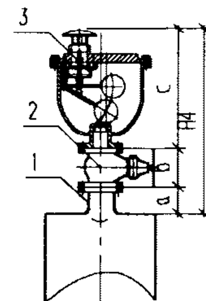
CARX复合排气阀乙型安装
